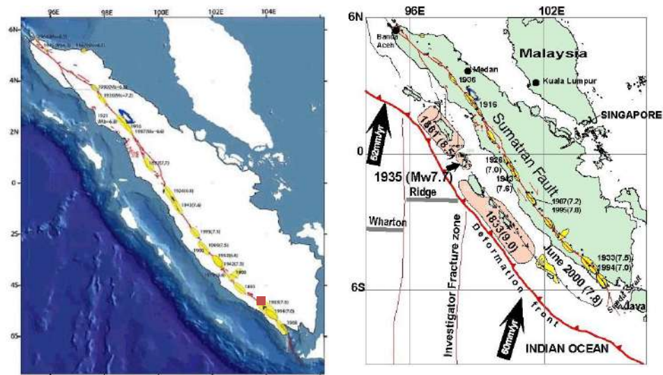
Gambar II. 8 Sesar Semangko dan Subduction Zone
